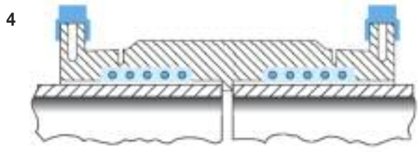
4 Area of melt extends leading to expansion towards pipe surface.
