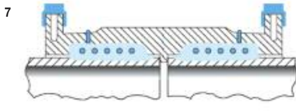
7 Melt pressure reaches optimum value at end of energising cycle. Emergence of the melt at the indicator holes shows that fusion is complete.
