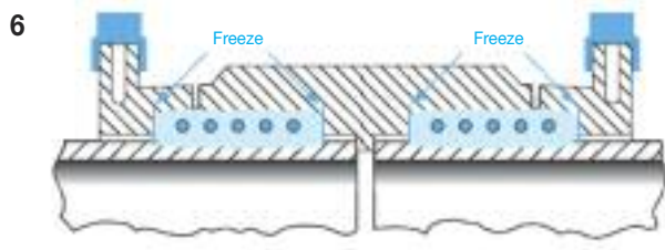
6 Melt solidifies at the start of the cold zones, thereby sealing the melt zone. Further input of energy causes increase in melt pressure.
